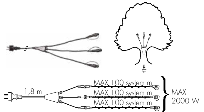
484-23 3000 TREE - START SYSTEM EXPO
